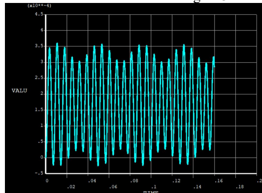
Figure 2. Finite Element Calculation Results of Displacement Time History Response of Lower Fixture Mass Block
