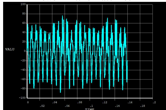
Figure 3. Finite Element Calculation Results of Acceleration Time History Response of Lower Fixture Mass Block
